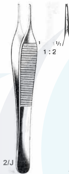
ADSON 56-694 12 CM 1x2 Teeth
