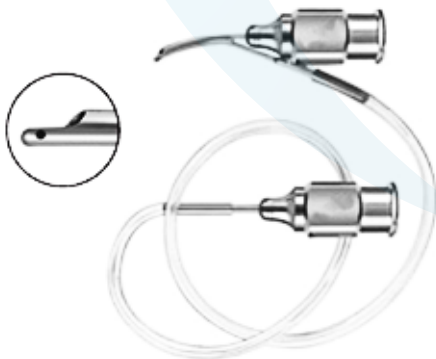
56-0480 SIMCOE 15 MM LONG 0.3MM DIAMETER ASPIRATION PORT
